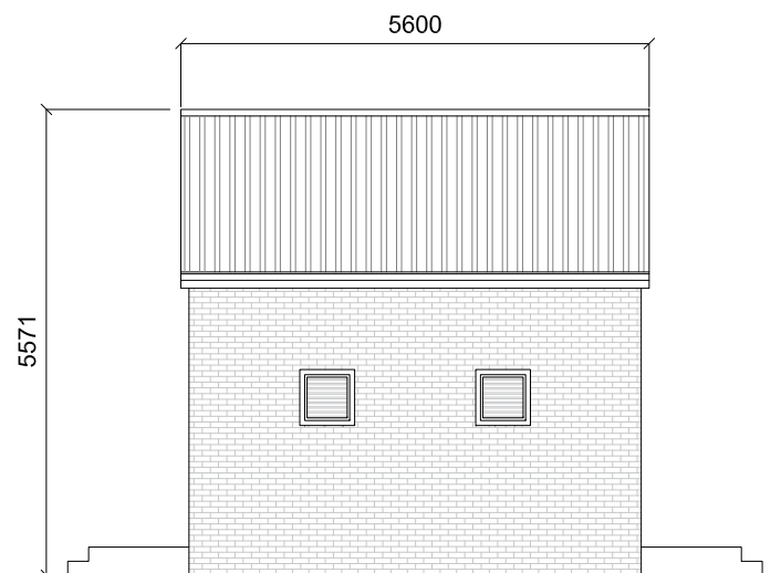
SIDE ELEVATION
